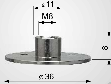
30990-0750 shelf plate Bodenplatte supporte de tablettes large /
