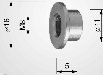
30990-0710 shelf holder 5 mm Bodenhalter 5 mm support de tablettes 5 mm
